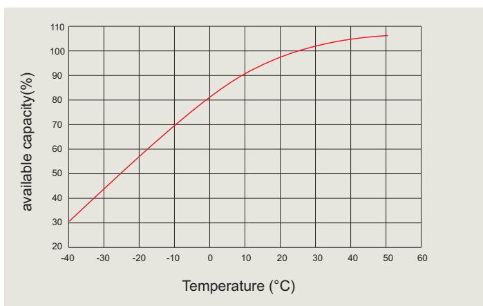
Available Capacity (10h rate and Voltage 1.80V) VS Ambient Temperature
