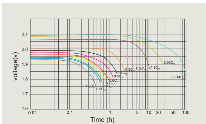
Discharge performance Curves at Different Discharge Rates(25°C)
