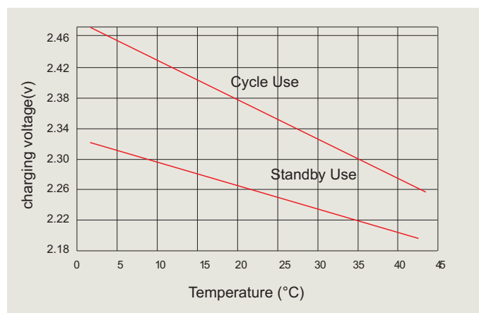
Float Voltage/Equivalent Voltage VS Temperature
